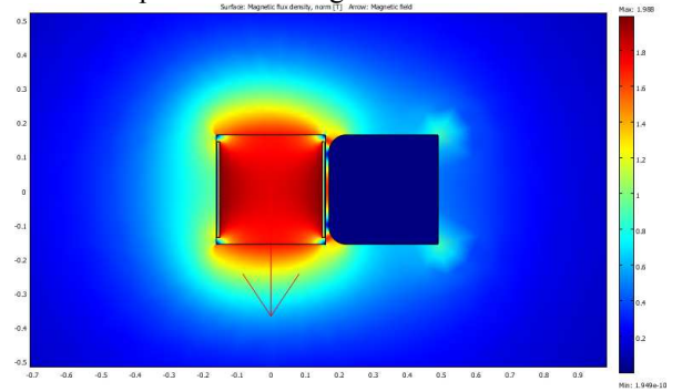
FIGURE 4. The 2D design of the SC septum.
